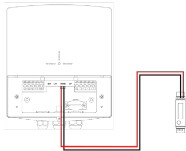
EV to GEM120CT comms
