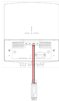
EV to EM115 comms
