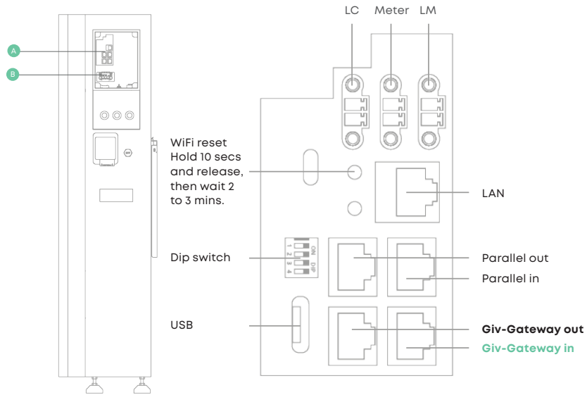
All in One Communication / Network Ports
